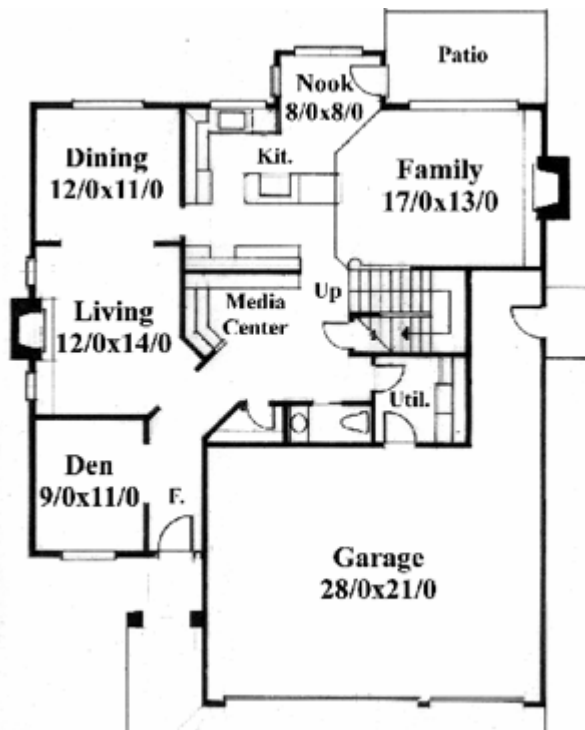
P lan M-2719 43/0 wide x 54/0 deep 2,719 sq. ft.
