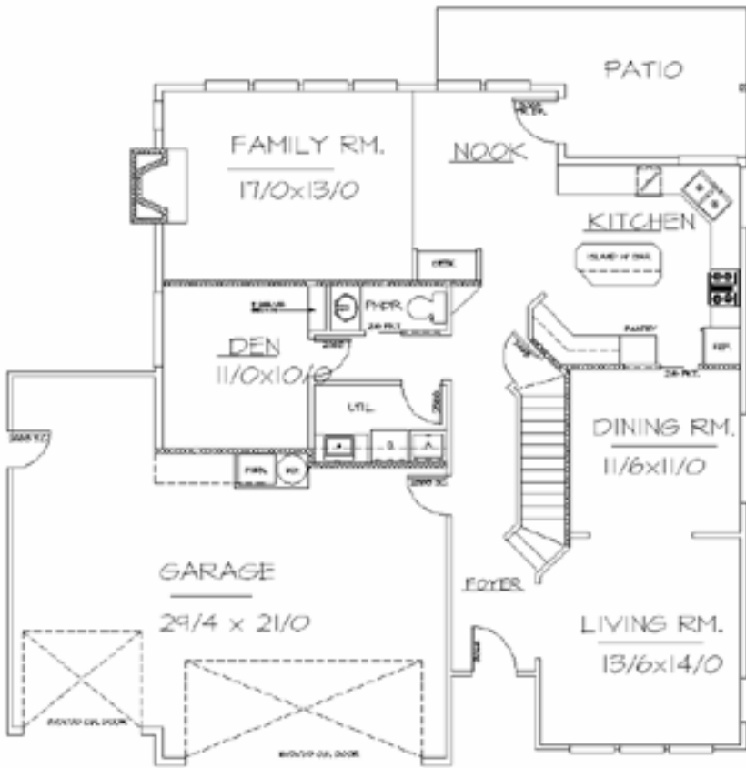
P lan M-2662 50'0" wide x 46'0" deep 2,662 sq. ft.
