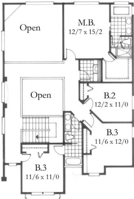
Plan M-2501fr 38/0 wide x 52/4 deep 2501 sq. ft.
