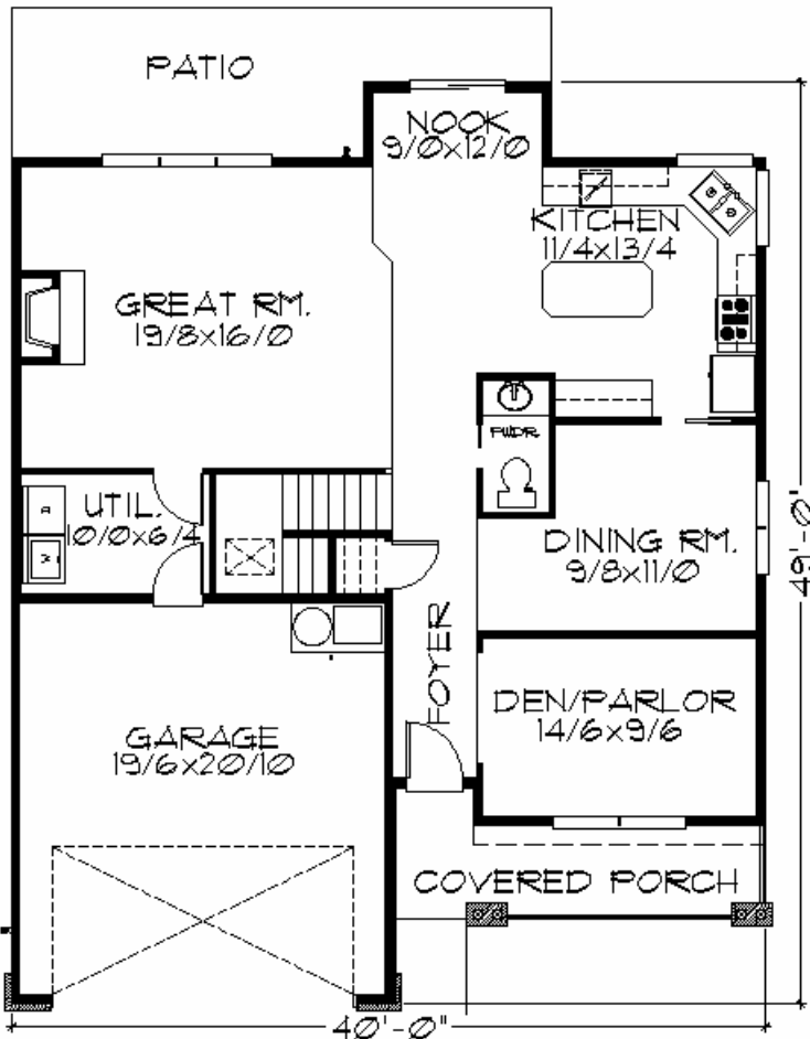
P lan M-2226 40/0 wide x 49/0 deep 2,227 sq. ft.
