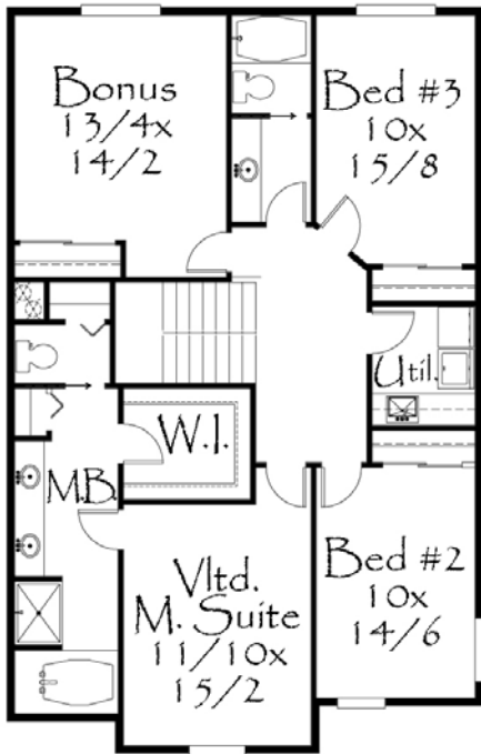
Plan M-2204GF 30/0 wide x 50/0 deep 2204 sq. ft.
