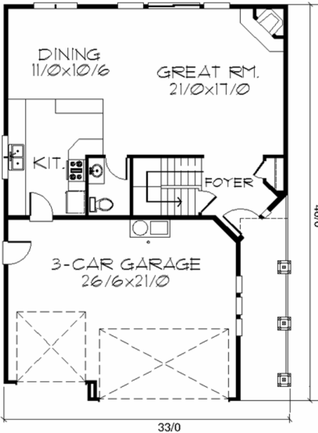
Plan M-2165 33/0 wide x 46/0 deep
