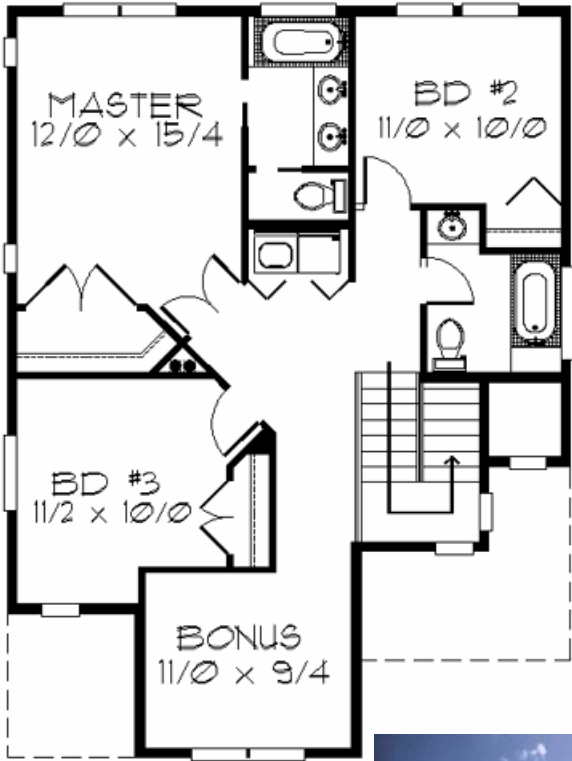
Plan M-1689 30/0 wide x 40/0 deep 1,689 sq. ft.
