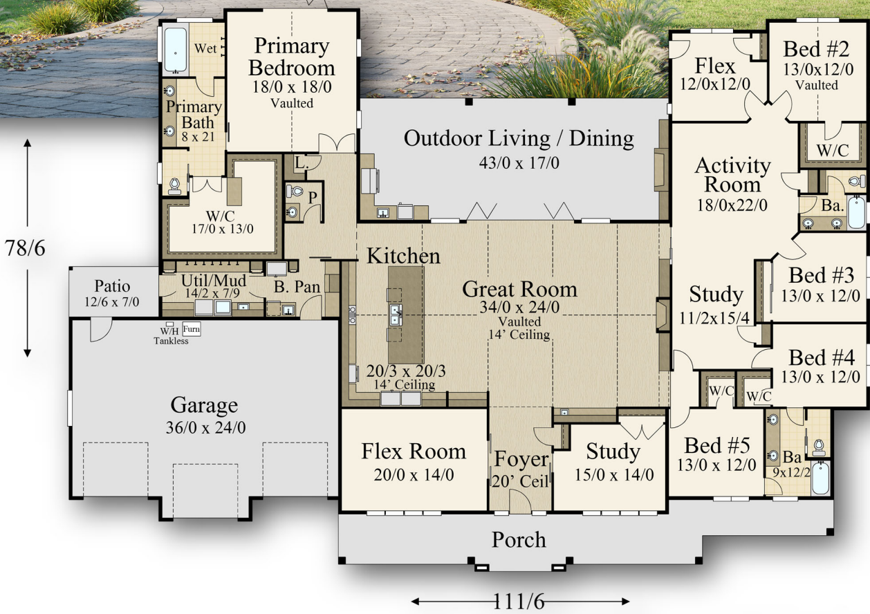
Main Floor - 4,841 Sq. Ft.
